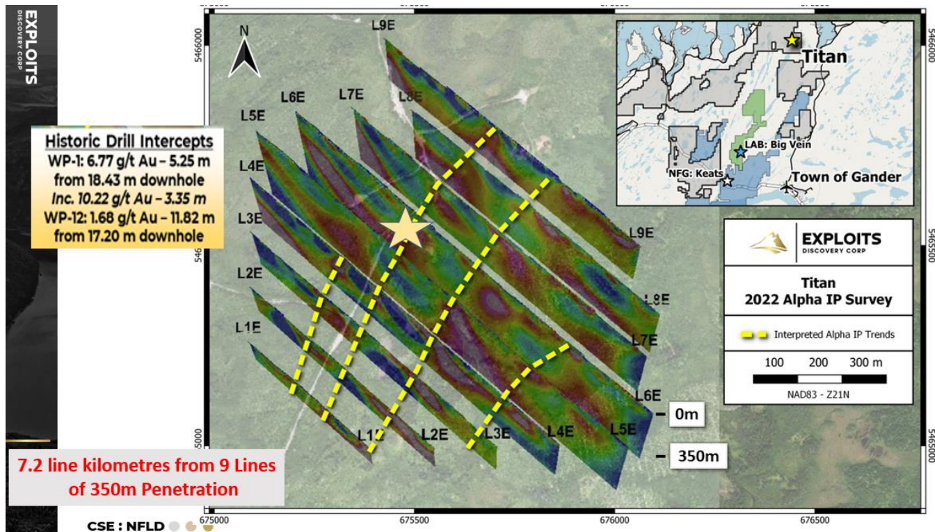
Fig. 4: Vertical IP profiles with the Titan area derived from the 2022 Alpha IP geophysical programme.
