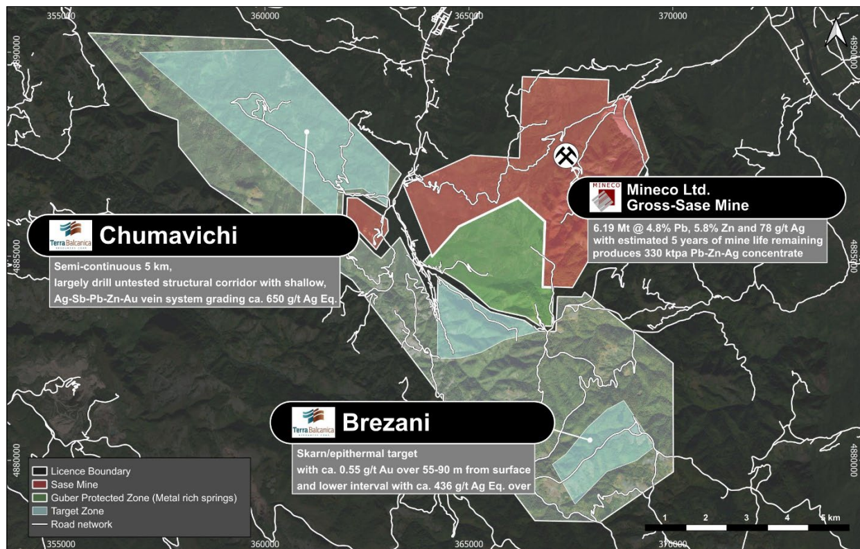
Figure 1. The Viogor mineral exploration licence encapsulates the three mineralized localities which will be advanced over the next 7 years. The operating Mineco Ltd. Sase mine is strategically located 7 and 11 km away from Čumavići and Brežani, respectively ( click here to view image ).
