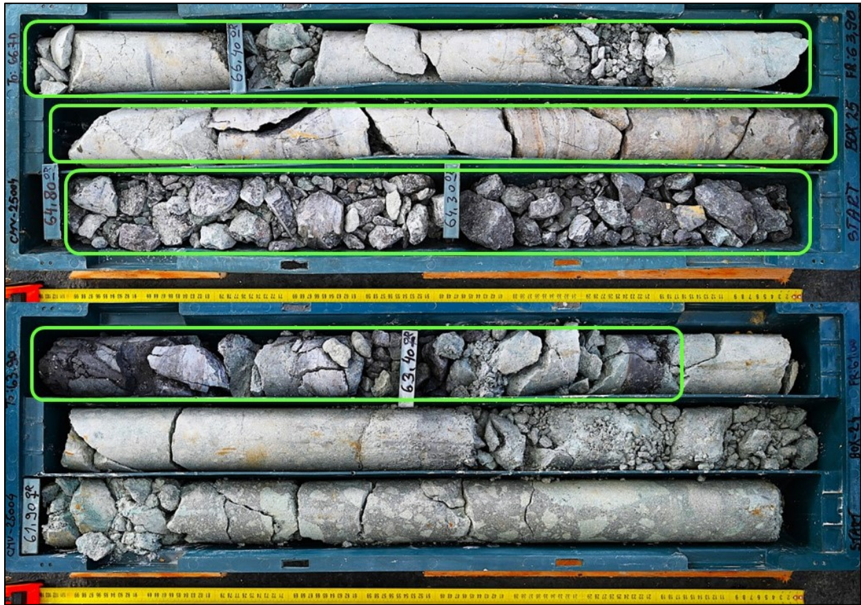
Figure 1. Photograph of PQ3 diameter core between 61.0 and 66.70 downhole in CMV25004. Massive, dark sulphide intervals can be observed in the lower box, correlating to the Ag-Sb mineralization while banded honey brown segment in the central part of the upper core box indicates Zn-Pb rich zone ( click here to view image ).
