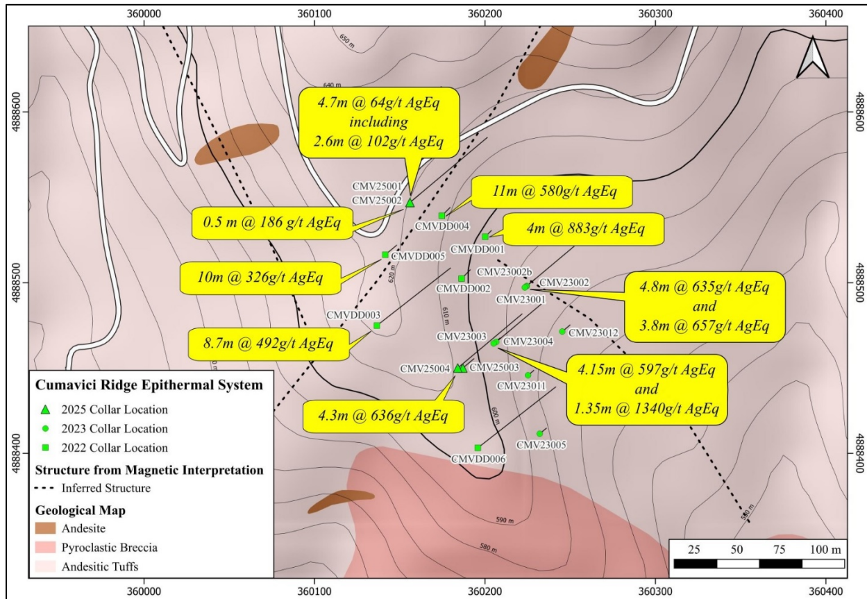
Figure 2. Geological map illustrating the drillholes at the Cumavici Ridge locality. AgEq values are labelled for selected 2022 and 2023 drill intercepts (See Company’s new releases dated 13 November 2023, 27 February 2023). The coordinate reference system is WGS84/UTM Zone 34N ( click here to view image ).
