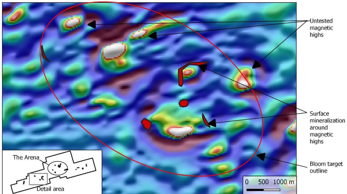
Figure 1. The Bloom Target overlain on a 1 st vertical derivative magnetic map. Several magnetic highs are untested.
