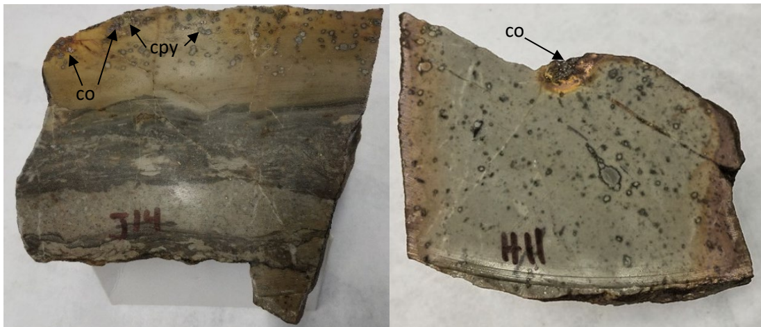
Figure 2. Photos of stratabound blebs of cobaltite (co) and chalcopyrite (cpy) with carbonate-hematite alteration in carbonate-mud rock of the East Cu-Co showing. Both rock samples are approximately 15 cm wide.
