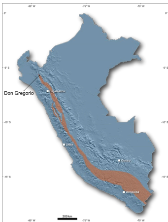
Figure 8. Location of the Don Gregorio Porphyry Cu-Au Project, Peru. The project is near the northern end of the Miocene magmatic belt (shown as an orange band), which is the host to large Miocene porphyry systems including Toromocho and Antamina.
