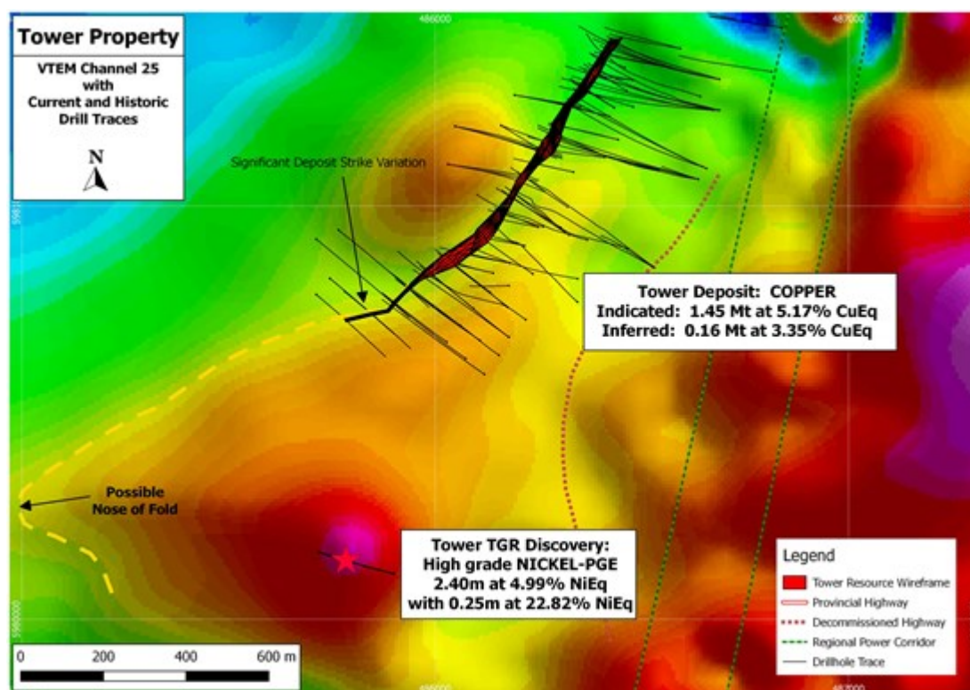
Figure 2: Tower TGR Ni-PGE Prospect
