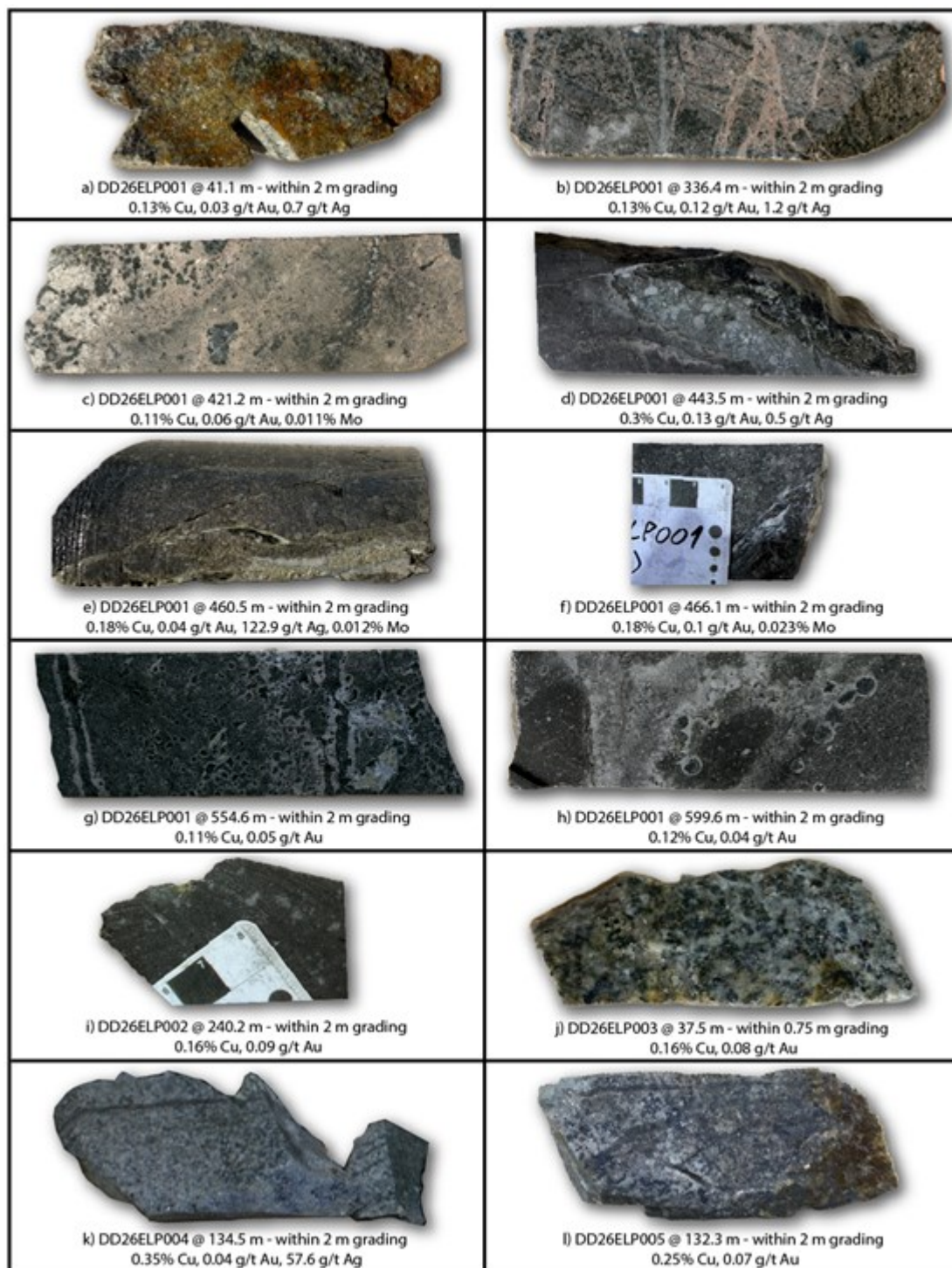
Figure 3 - Photographs of select drill core from 2026 diamond drilling at El Perdido. a) Partial replacement of pyrite-chalcopyrite by chalcocite in early-mineral diorite porphyry. b) Early-mineral quartz diorite porphyry with quartz-magnetite-pyrite-chalcopyrite stockwork veins and associated biotite-K-feldspar alteration. c) Early-mineral quartz diorite porphyry with evidence of localized high-temperature potassic alteration associated with early halo-type chalcopyrite-magnetite-quartz vein. d) Disseminated and vein-filling chalcopyrite with andesitic volcanics. e) Quartz-pyrite-chalcopyrite vein in biotite-chlorite altered andesitic volcanics. f) Quartz-chalcopyrite-magnetite vein in biotite weak potassic altered andesitic volcanics. g) Pyrite-chalcopyrite associated with orthoclase alteration in andesitic volcanics. h) Pyrite-chalcopyrite associated with orthoclase alteration in andesitic volcanics. i) Coarse chalcopyrite within biotite-chlorite altered andesitic volcanics. j) Fracture-controlled chalcocite replacement of pyrite-chalcopyrite within early-mineral diorite porphyry. k) Fracture-controlled chalcocite replacement of pyrite-chalcopyrite in sheeted quartz veins. l) Early-mineral quartz diorite porphyry with partial chalcocite replacement of pyrite and chalcopyrite in quartz stockwork veining.
