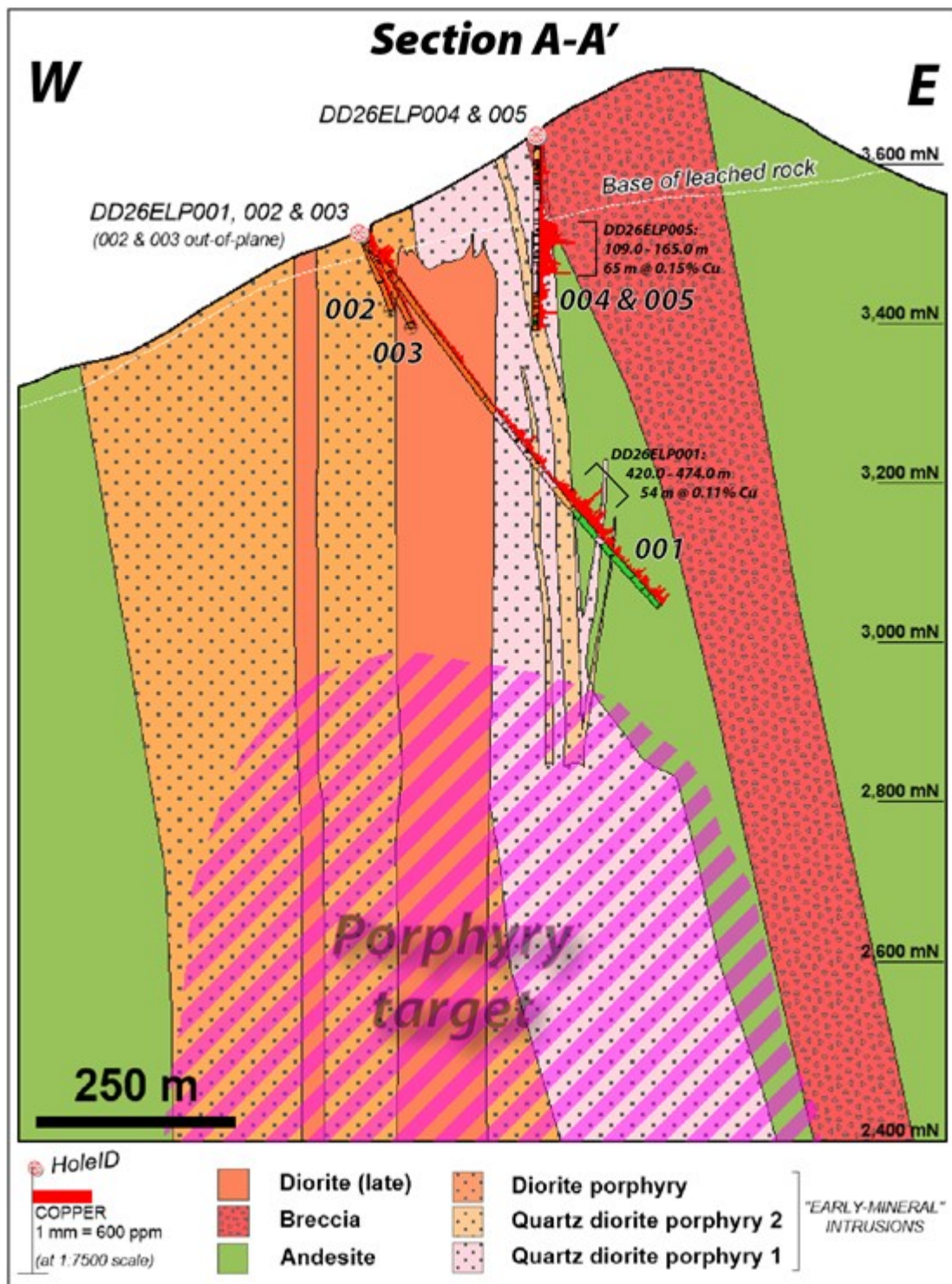
Figure 2 - Geological cross-section interpreted from 2026 diamond drilling results at El Perdido showing core of porphyry system at depth.
