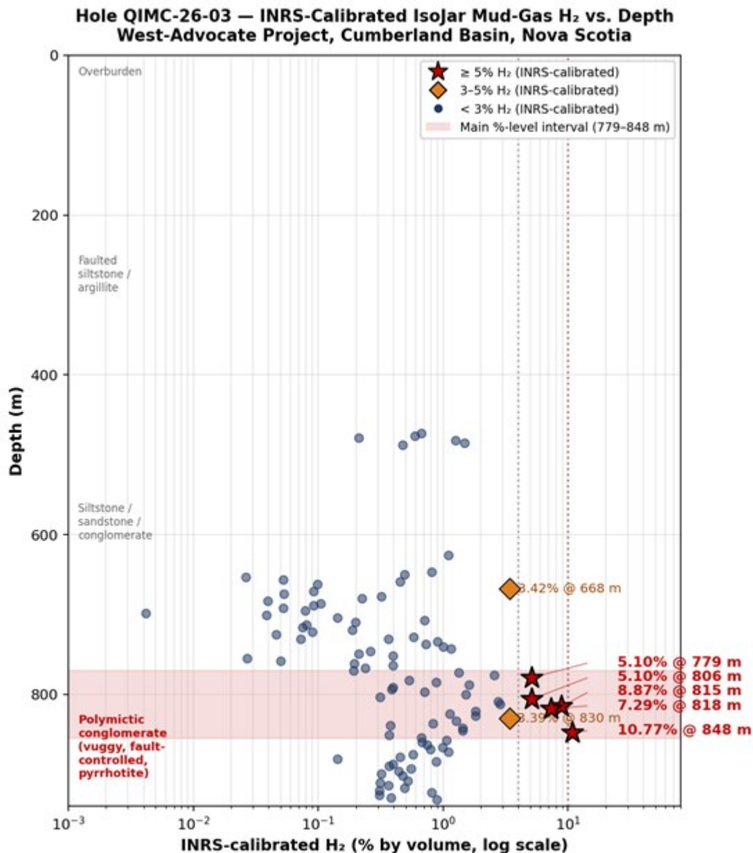
Figure 1. Depth-concentration profile of all 102 IsoJar H 2 mud-gas samples from QIMC-26-03. Red stars are the five readings ≥5% H 2 in the main %-level interval (779-848 m): 5.10% at 779 m, 5.10% at 806 m, 8.87% at 815 m, 7.29% at 818 m, and 10.77% at 848 m. Orange diamonds are the two readings between 3% and 5% H 2 (3.42% at 668 m and 3.39% at 830 m). Blue dots are all remaining readings below 3% H 2 . The shaded zone marks the main %-level interval hosted within vuggy polymictic conglomerate. Dotted vertical lines mark the LEL of H 2 in air (4% v/v) and 10% v/v.
