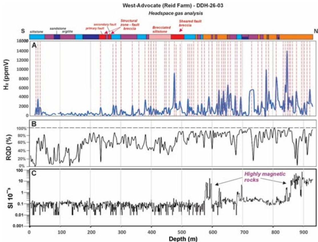
Figure 2. (A) Variability of H 2 concentrations (ppmV) measured in the water-headspace samples from drill hole DDH-26-03. (B) Rock Quality Designation (RQD, %) measured along the drill core. (C) Magnetic susceptibility values (SI × 10 -3 ) obtained from systematic core measurements.
