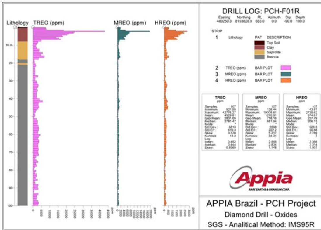
Figure 1 - Strip log of DDH PCH-F01R
